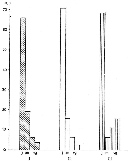
Fig. 1. Ages spectrums of populations I — STOROZHNTSA, II — KHOLMETS, III — ONOKOVTSY j — g — indexes of age states
