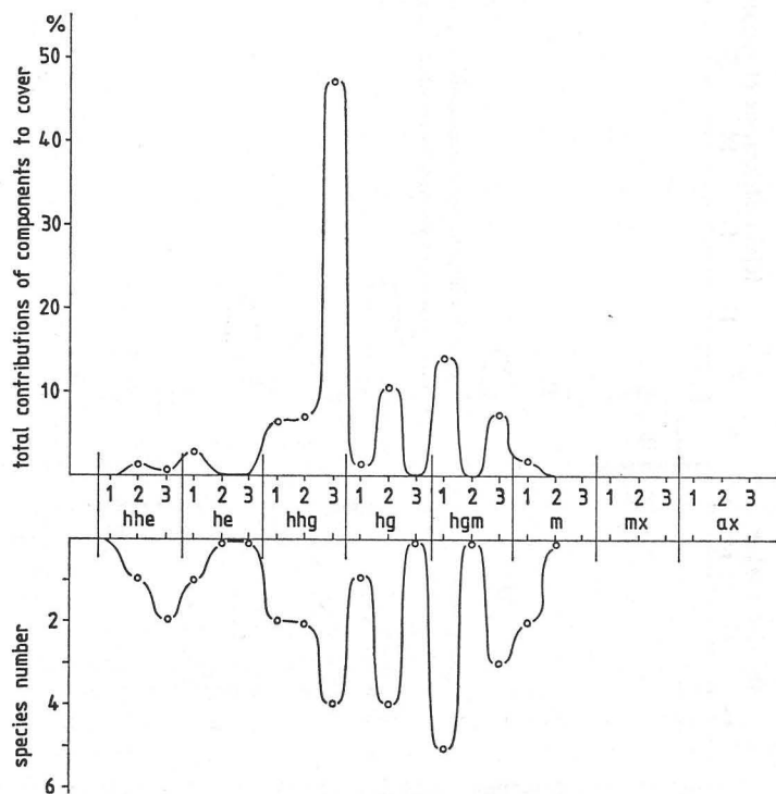
Fig. 6. Curve of the association drawn on the basis of the data reported by KÁRPÁTI et al. from the Middle Danube valley
