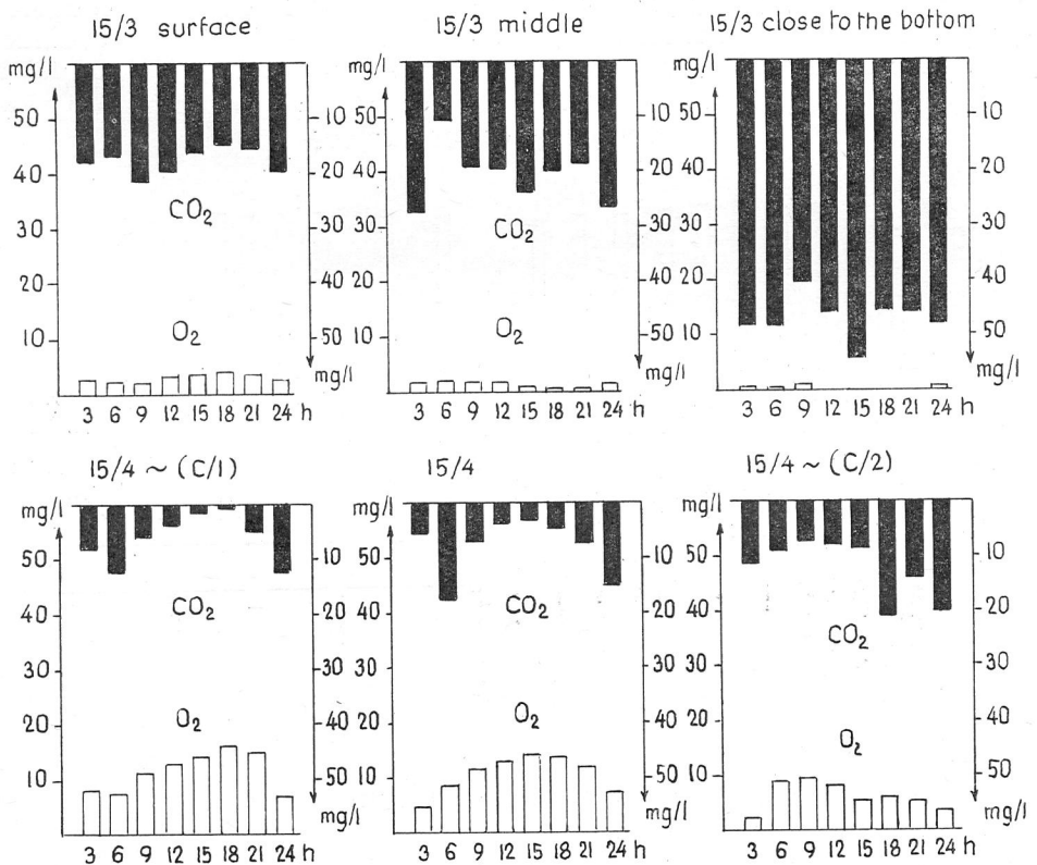
Fig. 4. Change in the quality of the dissolved O 2 and free CO 2 , according to the part of the day on August 5, 1975.
