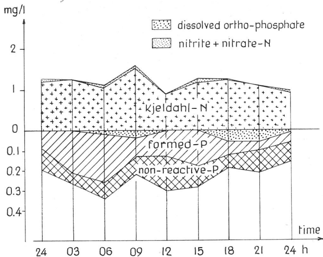
Fig. 2. Change in the quality of the nitrogen and phosphorus forms in the surface layer of open water, on September 17, 1974.
